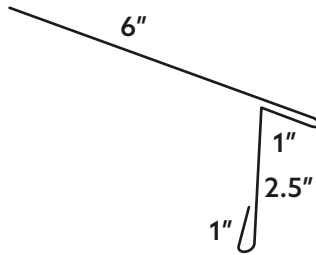
#407 - Upper Transition Drip Edge
