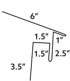
#406 - Hidden Fastener Upper Transition
