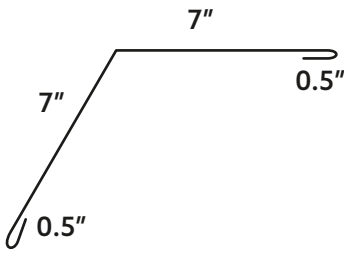
#401 - Ridge Cap
