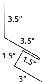
#418 - Head Wall with J Trim
