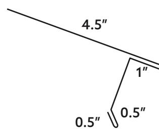
#408A - Roof Drip Edge
