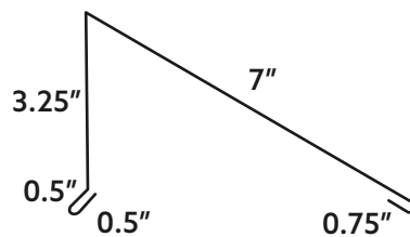
#414A - Half Ridge Cap
