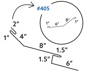
#404A - Hidden Fastener Transition
